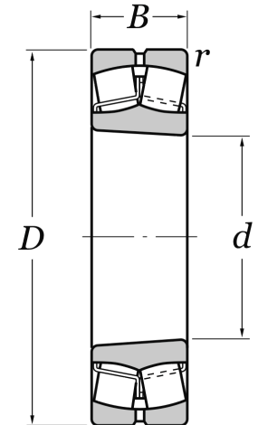
Tapered Bore
